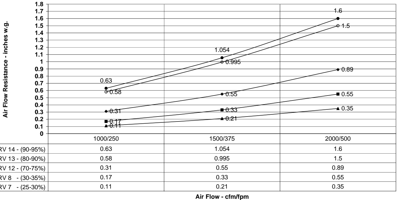
Resistance vs. Air Flow
