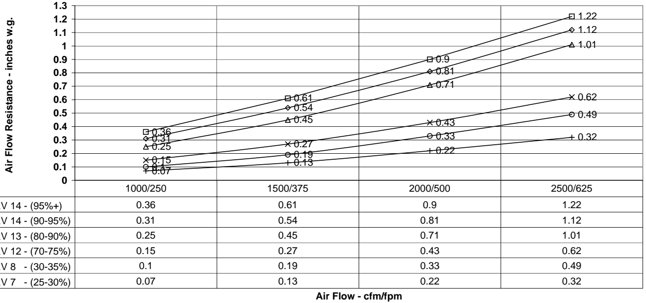
Resistance vs. Air Flow
